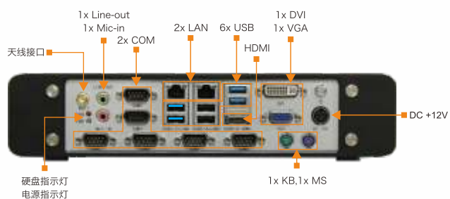
BIS-6660 C30接口
